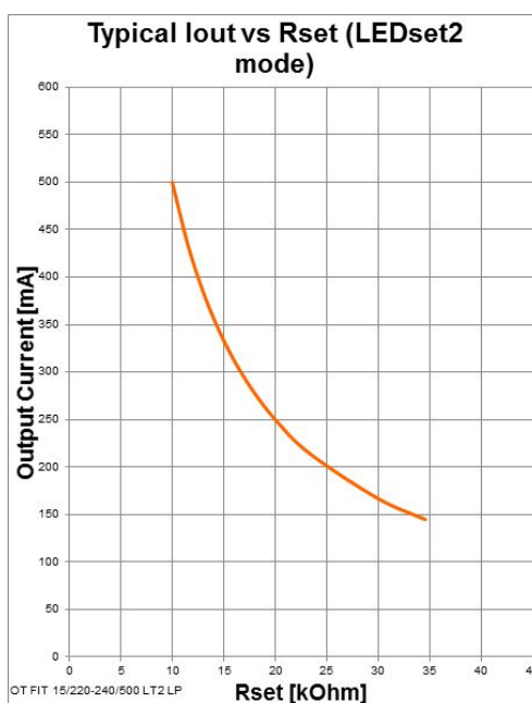
Typical Iout vs Rset (LEDset2 mode) OT FIT 15/220-240/500 LT2 LP
