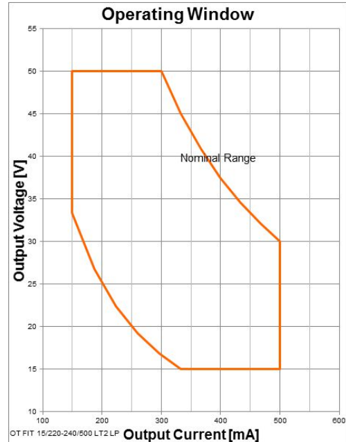
Operating Window OT FIT 15/220-240/500 LT2 LP
