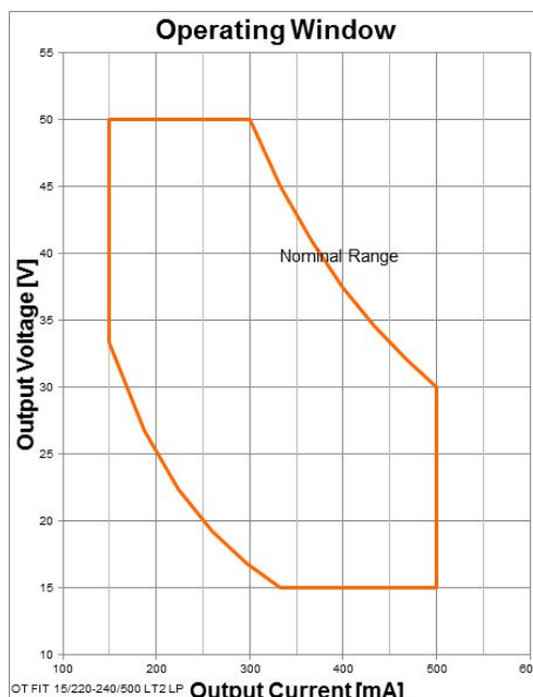
Operating Window OT FIT 15/220-240/500 LT2 LP
